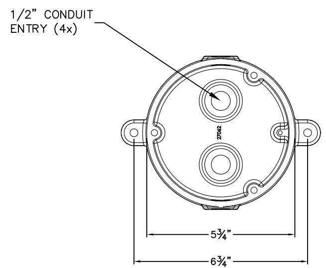
BACK BOX PLAN VIEW
