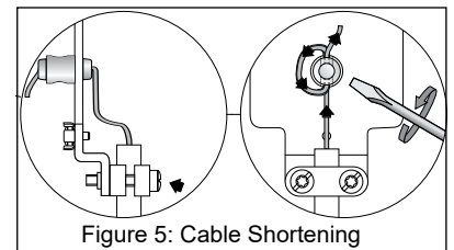
Figure 5: Cable Shortening
