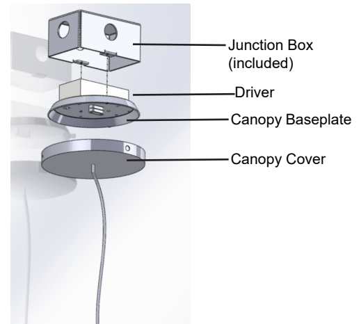
Figure 1: Mounting Canopy (Generic Image)
