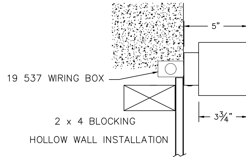
CONCRETE INSTALLATION
