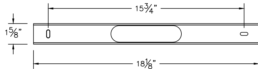
MOUNTING BRACKET
