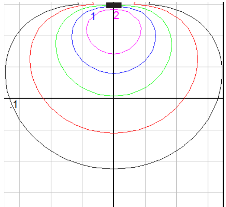
Wall Mount - Isofootcandle grid on floor Mounting Height = 5 ft. Grid Spacing = 5 ft.
