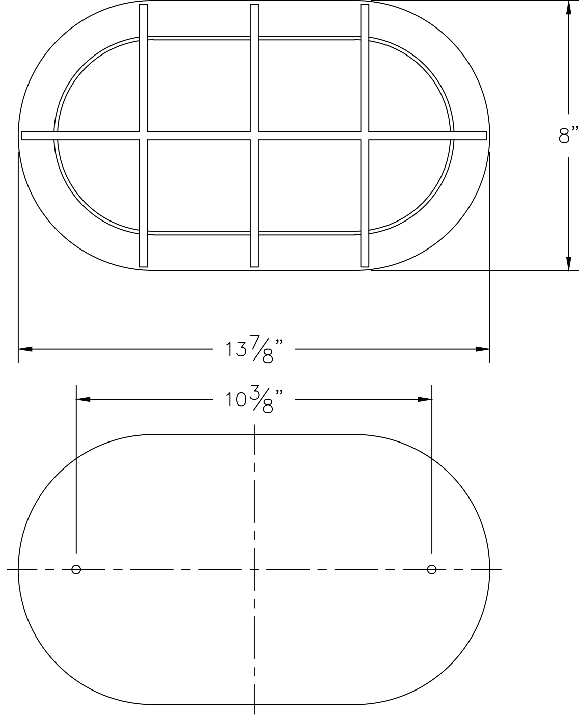
MOUNTING DETAIL
