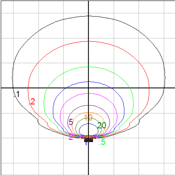
Wall Mounted Fixture - Iso-Grid on Wall Grid Spacing = 5 ft.
