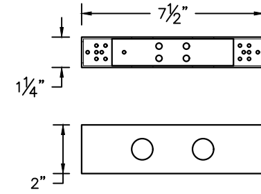
CUSTOM WIRING BOX DETAIL
