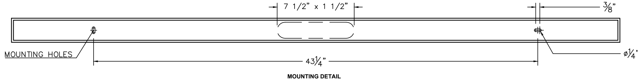
MOUNTING DETAIL
