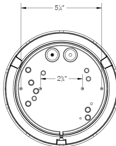
Figure 2: Luminaire back with round wall mount casting
