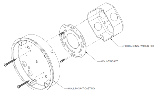
Figure 1: Mounting kit detail
