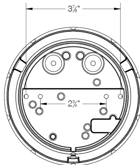
Figure 2: Luminaire back with round wall mount casting
