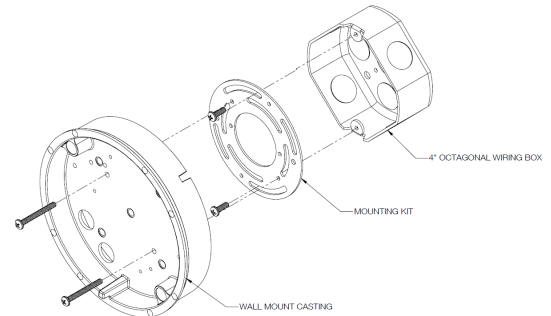
Figure 1: Mounting kit detail
