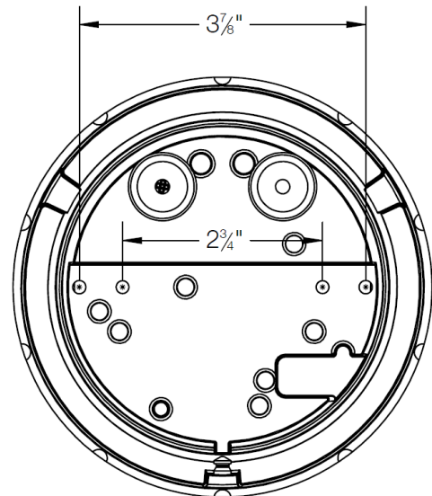
Figure 2: Luminaire back with round wall mount casting
