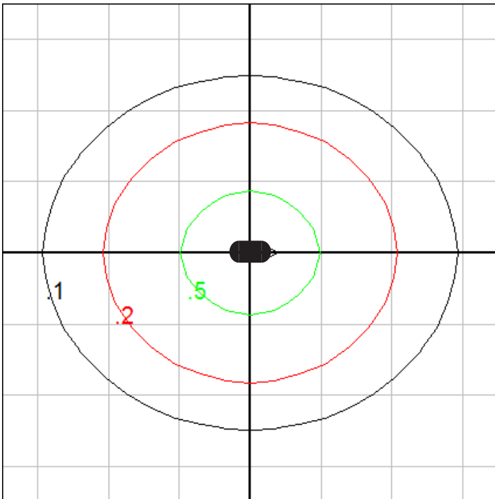
Ceiling Mount - Isofootcandle grid on floor Mounting Height = 5 ft. Grid Spacing = 5 ft.
