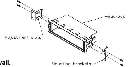
Figure 1 (stud wall)
