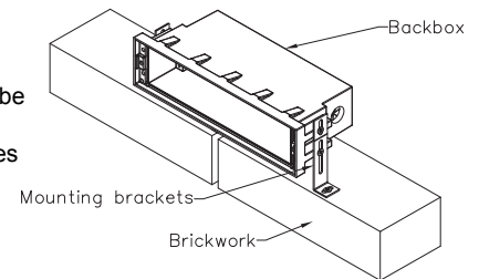
Figure 3 (brick wall)
