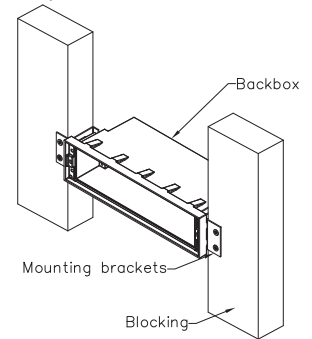
Figure 2 (stud wall)
