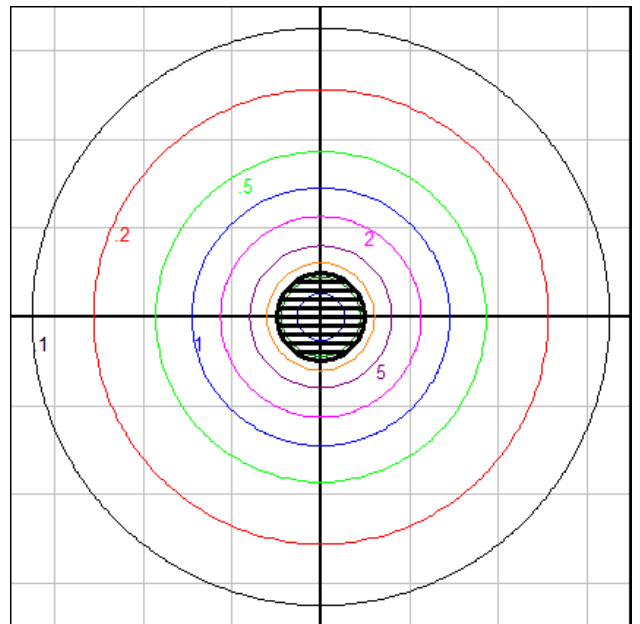
Wall Mount - Isofootcandle grid on wall Grid Spacing = 2 ft.
